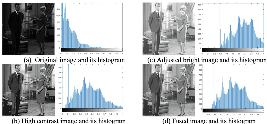
Fig. 5. Simulation results and their respective histograms of the Room image: (a) original, (b) high-contrast, (c) adjusted-bright, and (d) fused image.
